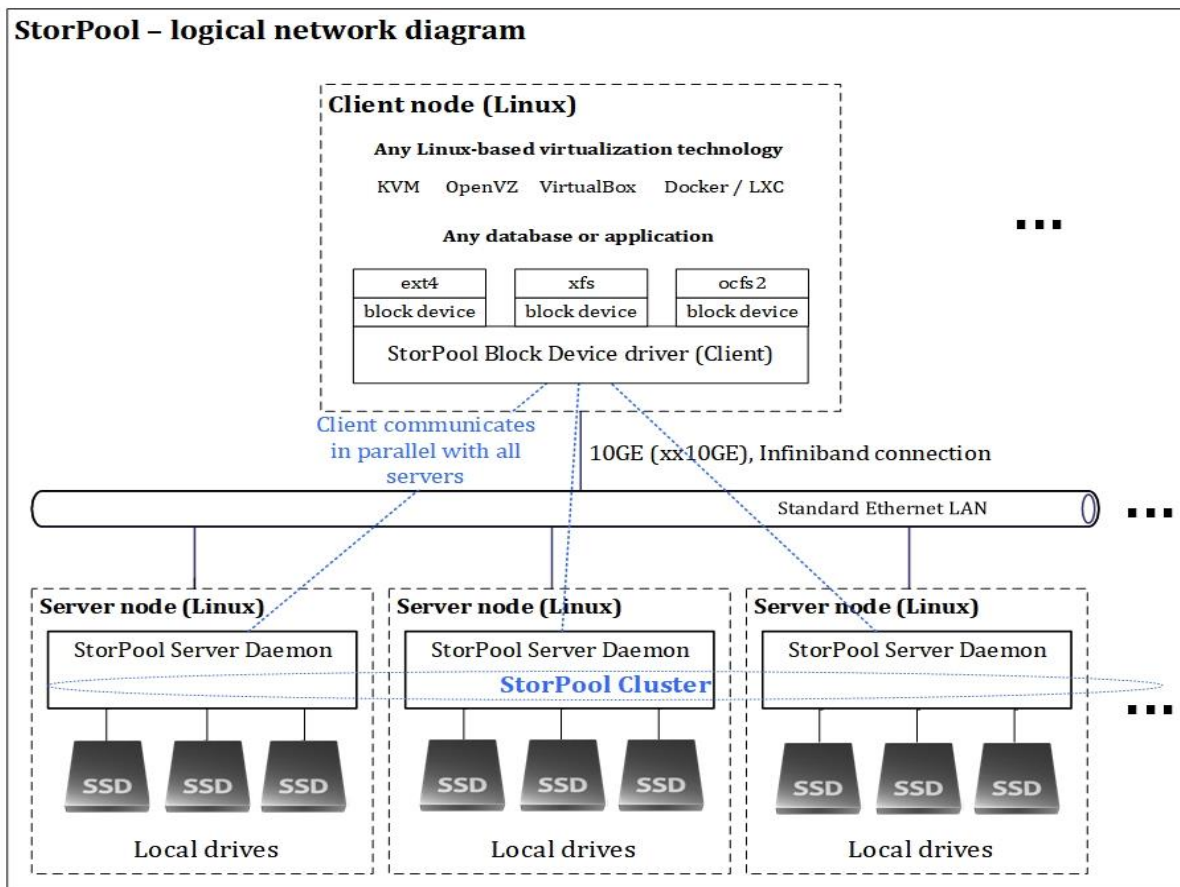
Fig. 2. Logical network diagram, stand-alone (storage on separate servers). We also support converged deployments - a StorPool Client & StorPool Server on the same physical server.
