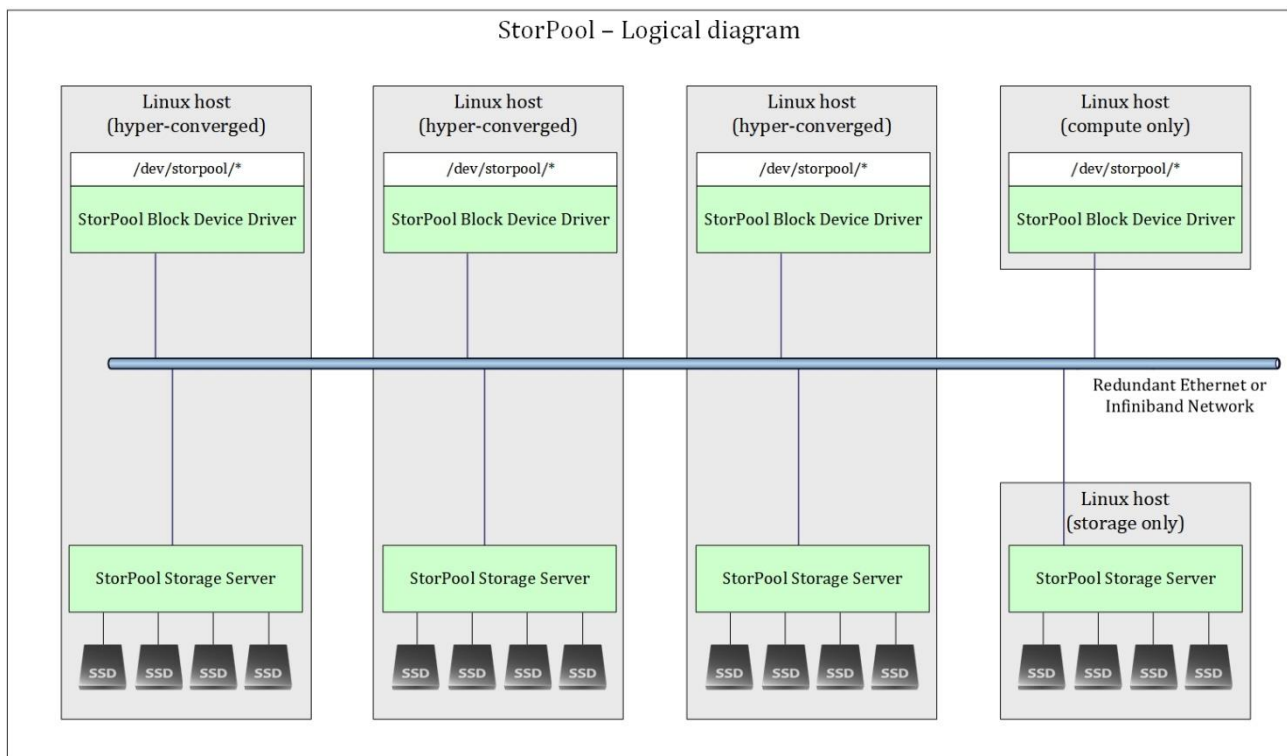
Fig 1. StorPool - Logical diagram
